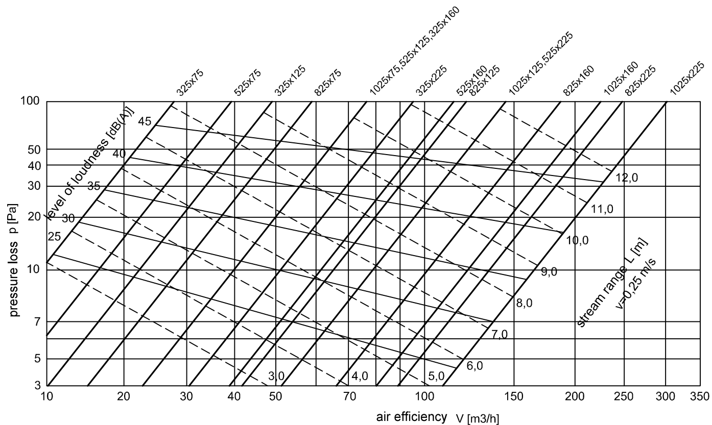
Diffusers NK/DZ
